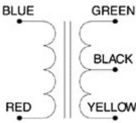
Schematic 2
