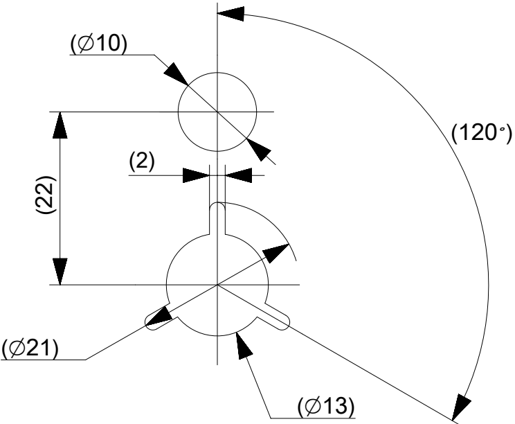
DETAIL "Z"
