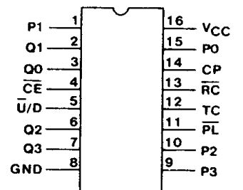
HC/HCT190, HC/HCT191 TERMINAL ASSIGNMENT
