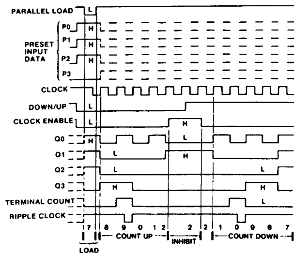
Fig. 4 - HC/HCT190 decade counters typical load, count, and inhibit sequences.
