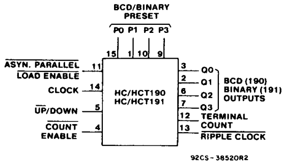
FUNCTIONAL DIAGRAM
