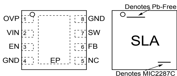
8-Pin MLF™ (BML) (Top View)
