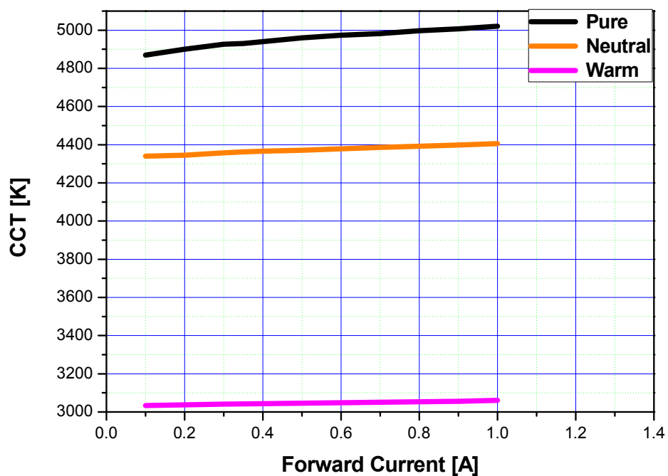
CCT vs. Forward Current, T_a=25^{\circ}\text{C}
