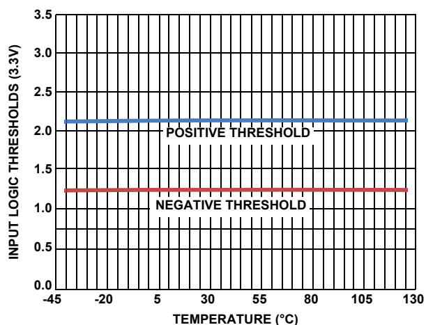
FIGURE 14. INPUT THRESHOLDS
