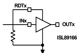
FIGURE 18. SETTING DELAYS WITH A RESISTOR
