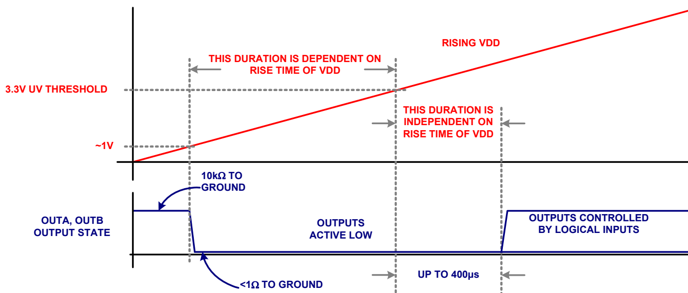
FIGURE 9. START-UP SEQUENCE
