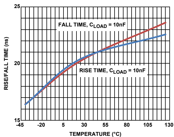
FIGURE 15. OUTPUT RISE/FALL TIME
