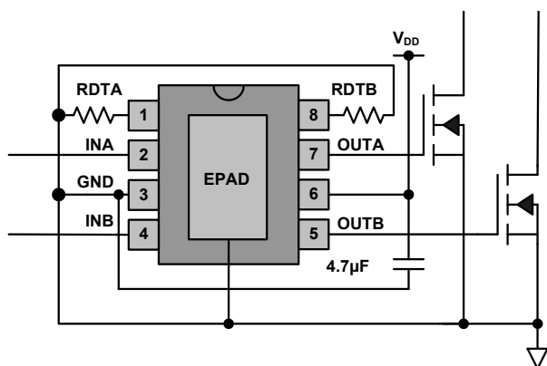
FIGURE 1. TYPICAL APPLICATION
