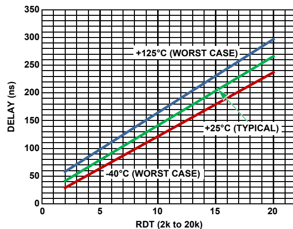
FIGURE 17. PROPAGATION DELAY vs RDT
