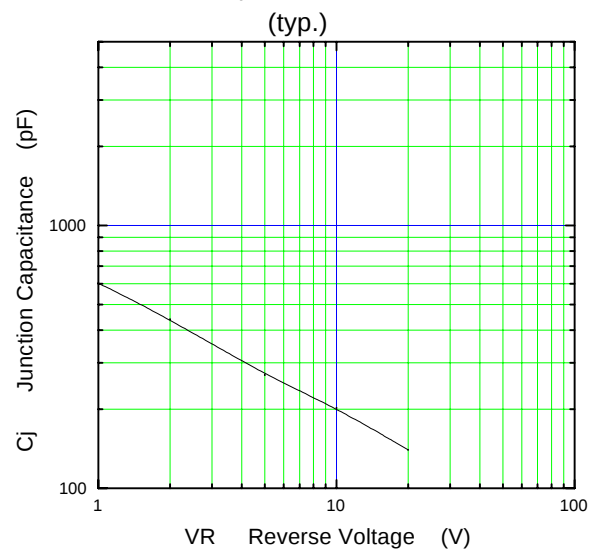
Junction Capacitance Characteristic
