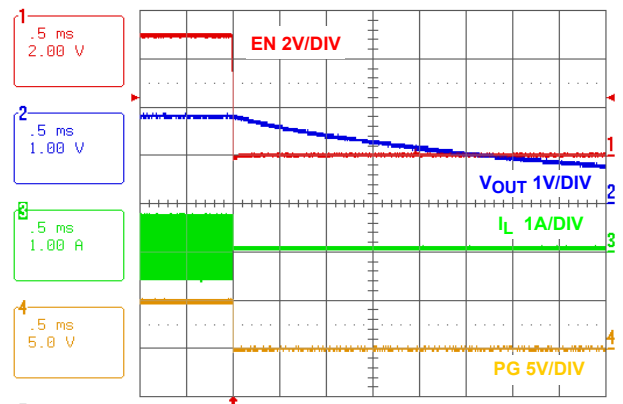
FIGURE 25. SOFT-DISCHARGE SHUTDOWN
