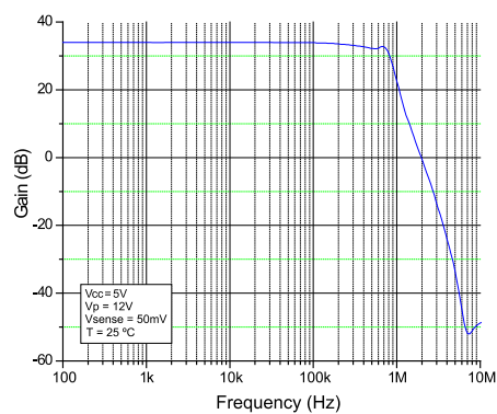
Figure 13: Bode diagram
