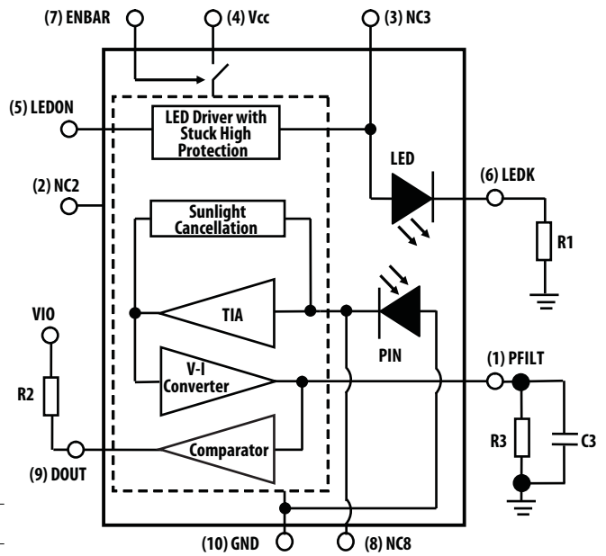
APDS-9120 Internal Block Diagram
