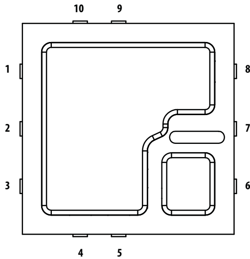
APDS-9120 I/O Pins Configuration Table
