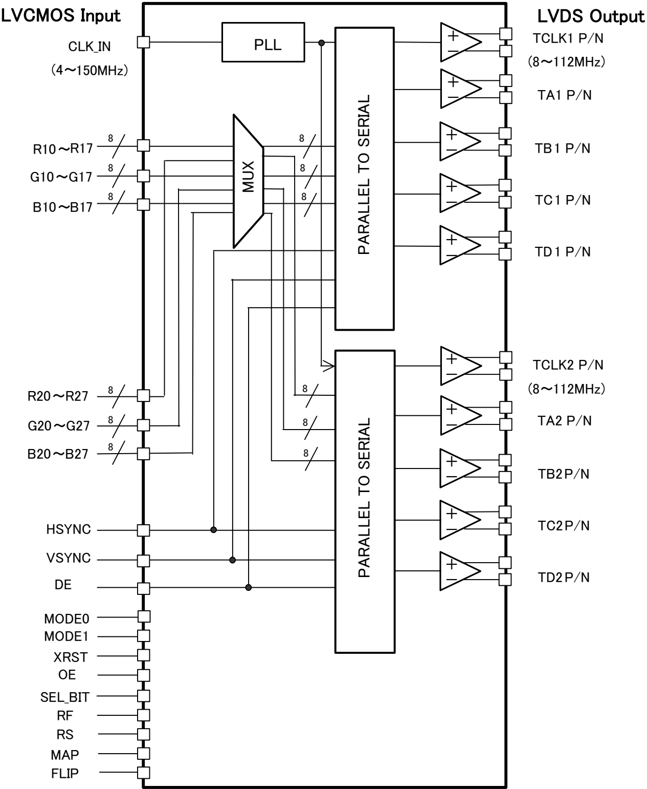
Fig.1 Block Diagram
