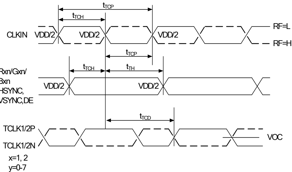
Fig.6 AC Timing Diagrams
