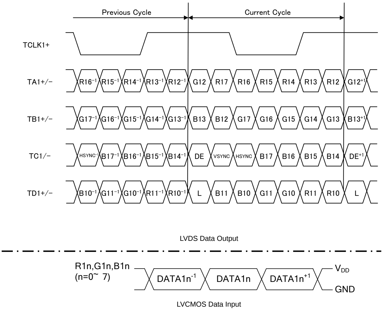
Fig.15 LVCMOS Data Inputs Timing Diagrams in Single Link
