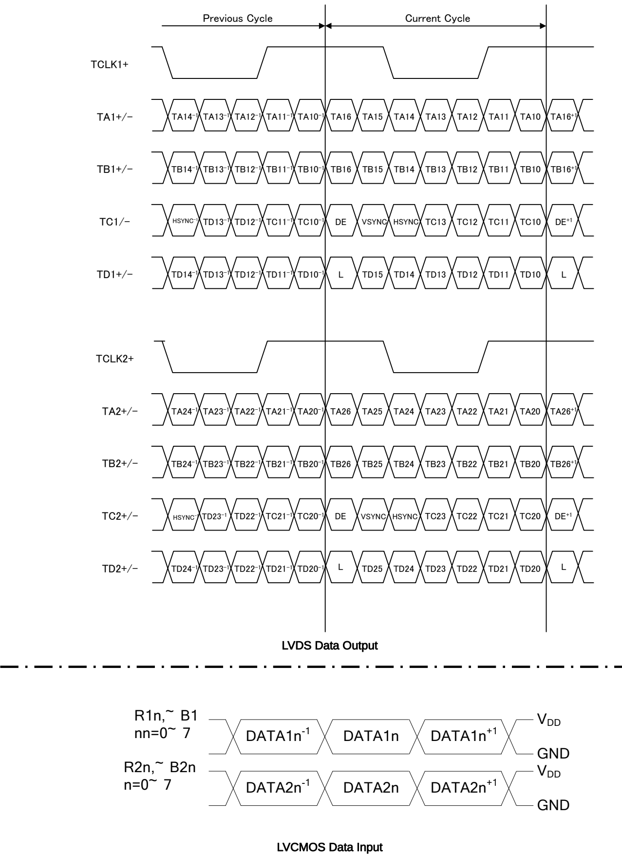
Fig.11 LVDS Output Data Mapping
