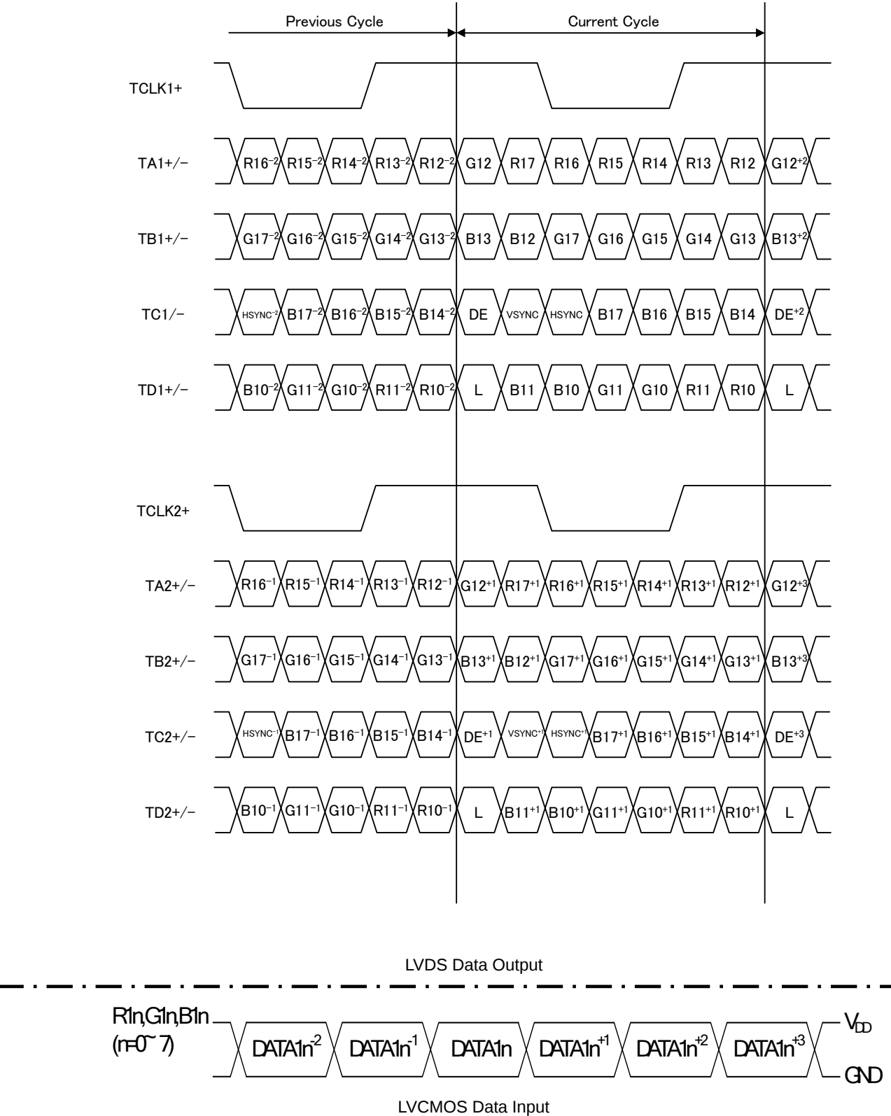
Fig.14 LVCMOS Data Inputs Timing in Dual Link
