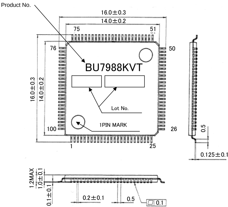
Fig.2 TQFP100V Package Outline and Specification
