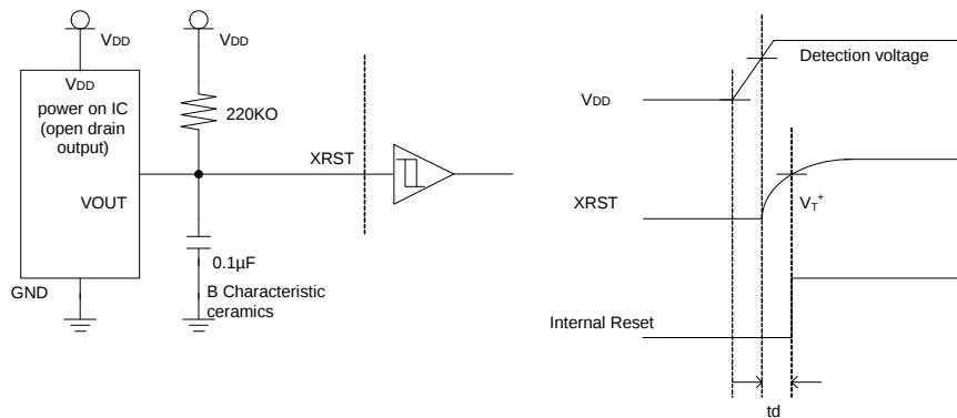
Fig.18 Power On Reset by specific
