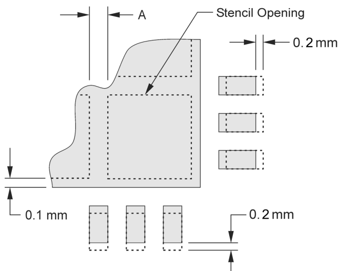
Figure 10-1. No Pullback WQFN, Single Row Reference Diagram
