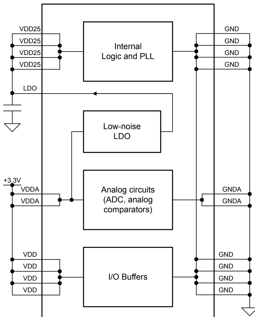
Figure 6-4. Power Architecture
