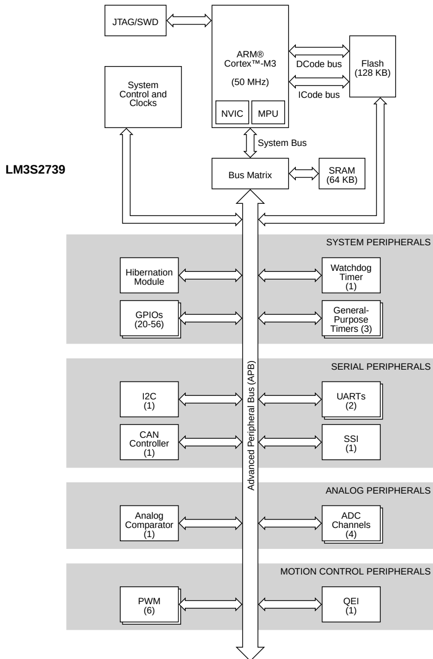
Figure 1-1. Stellaris® LM3S2739 Microcontroller High-Level Block Diagram
