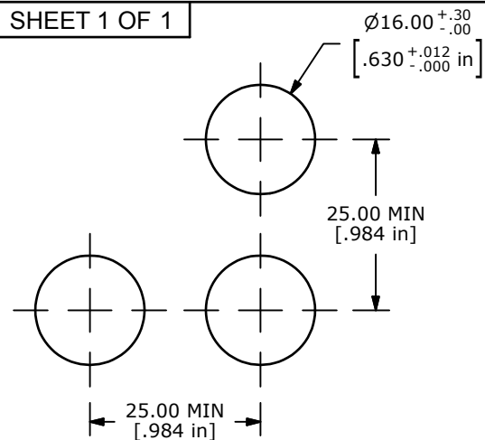
PANEL MOUNTING
