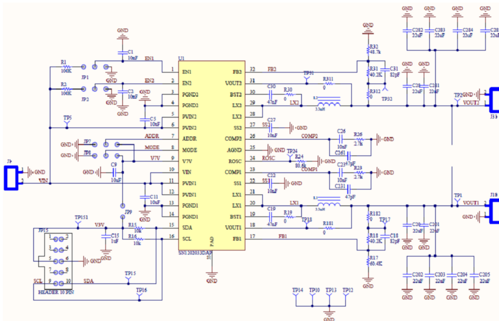
Figure 1. TPS65273V Schematic
