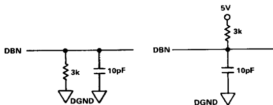
a. V_{OH} to High-Z
