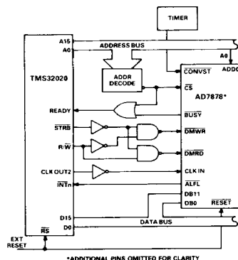
Figure 19. AD7878 - TMS32020 Interface
