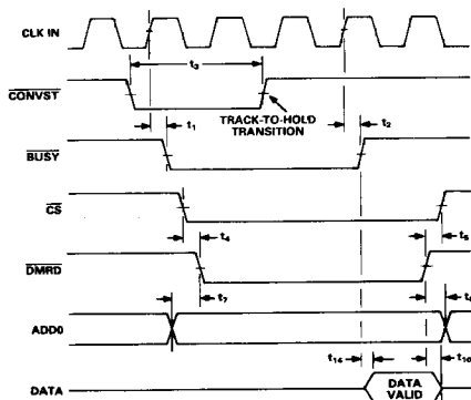
Figure 9. Extended Read Operation
