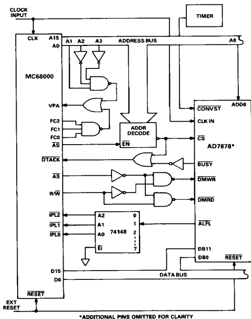
Figure 21. AD7878-MC68000 Interface
