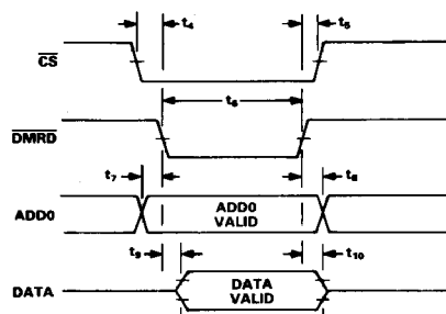
Figure 6. Basic Read Operation
