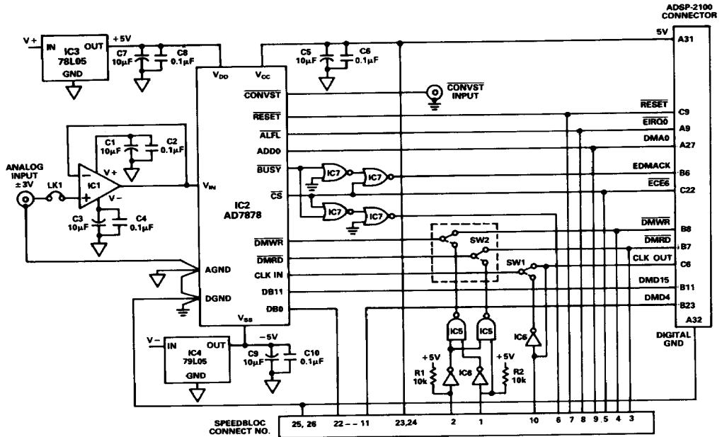
Figure 23. Data Acquisition Circuit Using the AD7878
