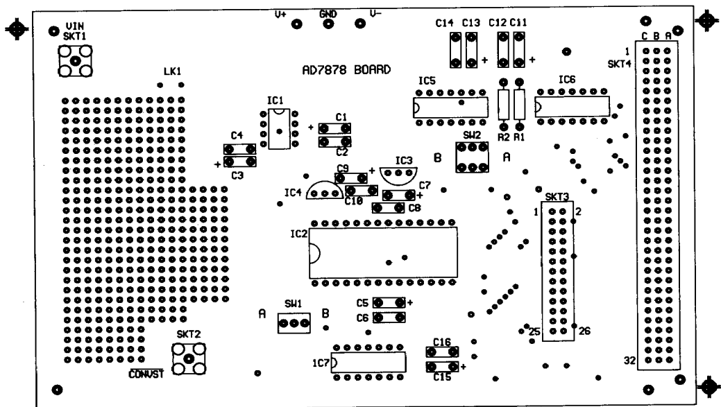
Figure 24. PCB Silkscreen for Figure 23
