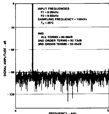
Figure 12. AD7878 IMD Plot
