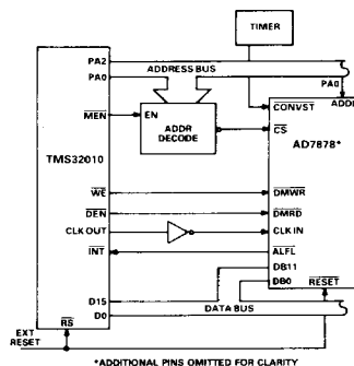
Figure 20. AD7878 - TMS32010 Interface
