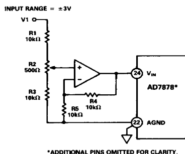
Figure 17. AD7878 Full-Scale Adjust Circuit
