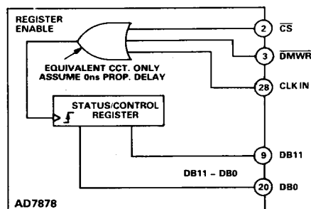
Figure 7. \overline{\text{DMWR}} Internal Logic
