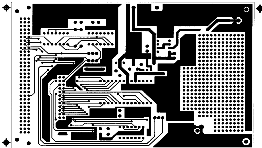
Figure 26. PCB Solder Side Layout for Figure 23
