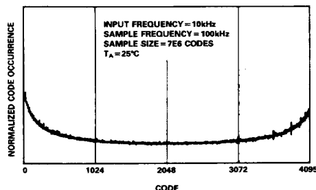
Figure 13. AD7878 Histogram Plot
