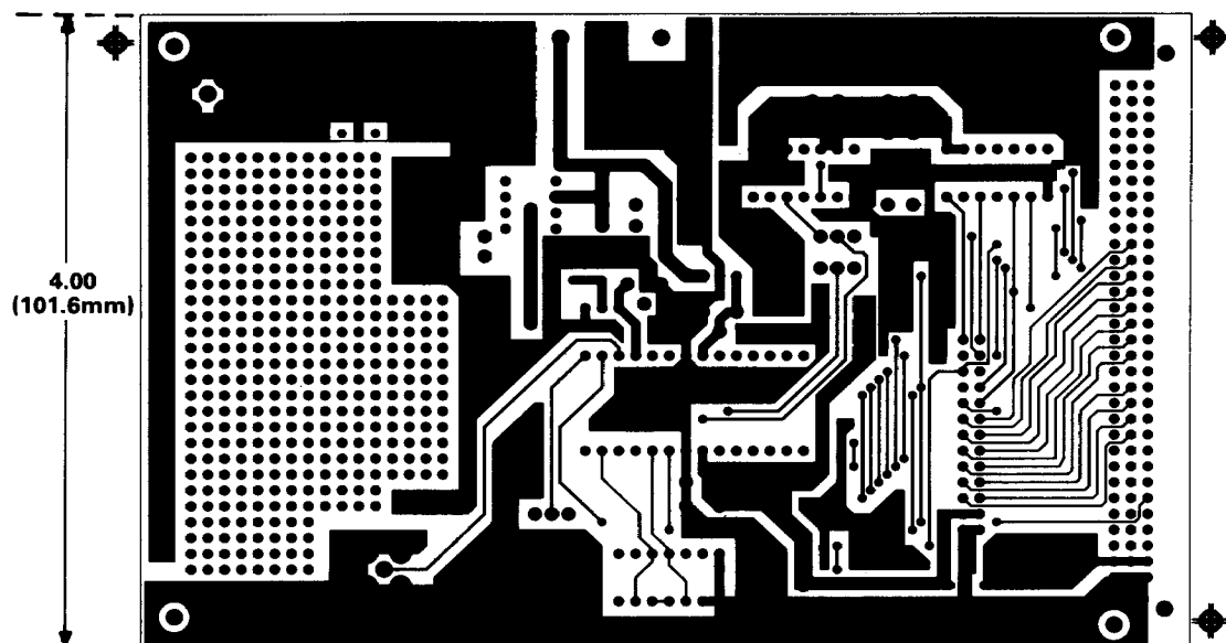
Figure 25. PCB Component Side Layout for Figure 23
