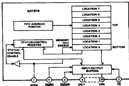
Figure 3. Internal FIFO Architecture
