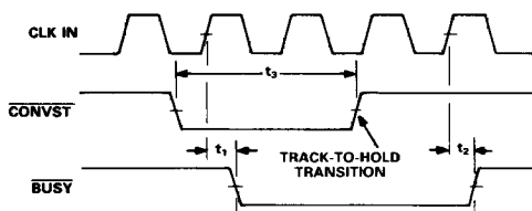
Figure 5. Conversion Start Timing Diagram
