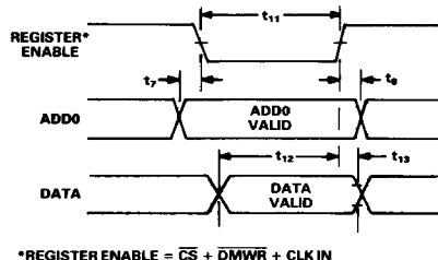
Figure 8. Basic Write Operation
