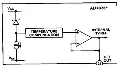
Figure 14. AD7878 Reference Circuit
