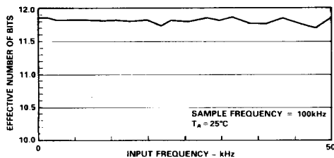
Figure 11. Effective Number of Bits vs. Frequency
