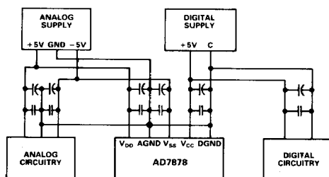
Figure 22. Power Supply Grounding Practice
