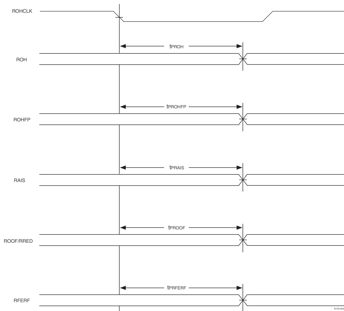
Figure 49 Receive Overhead Output Timing
