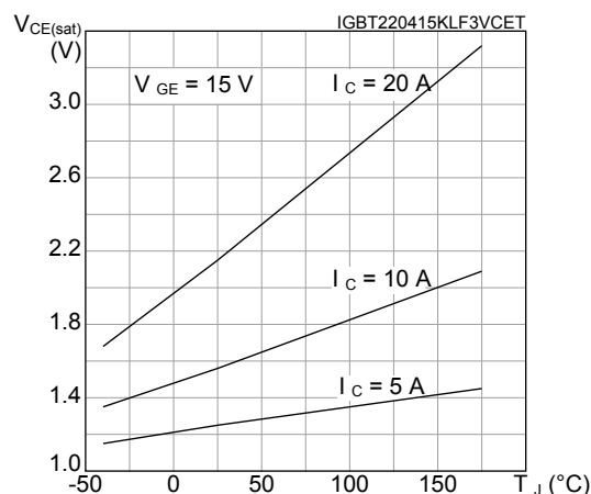
Figure 6. Typical V_CE(sat) vs temperature
