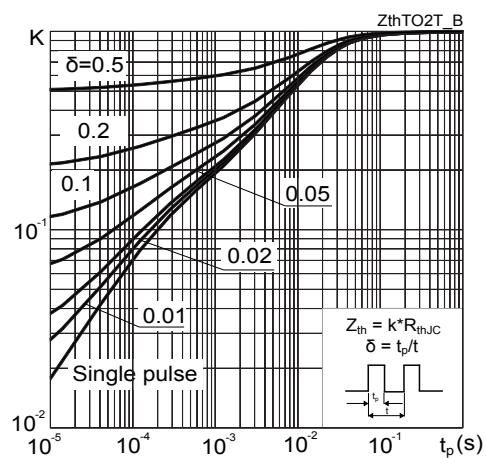
Figure 26. IGBT normalized transient thermal impedance
