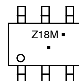
SC-88 CASE 419B-02
