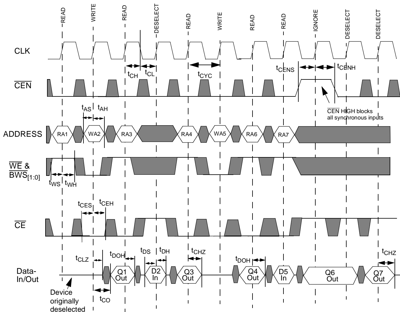
Read/Write/Deselect Sequence
