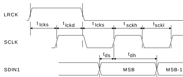
Figure 2. TDM Serial Audio Interface Timing
