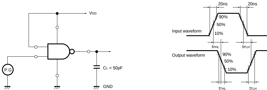
Fig. 2 Switching characteristics
