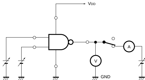
Fig. 1 DC characteristics
