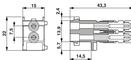
Dimensional drawing: VC-AFOS 2
