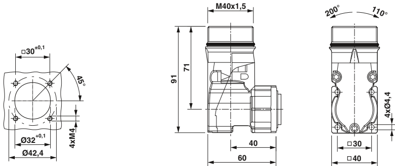
Installation dimensions
