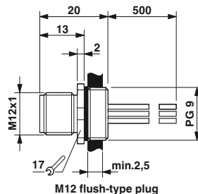
M12 flush-type plug
