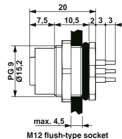
M12 flush-type socket
