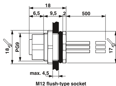
M12 flush-type socket
