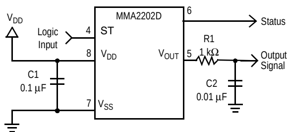
Figure 3. SOIC Accelerometer with Recommended
