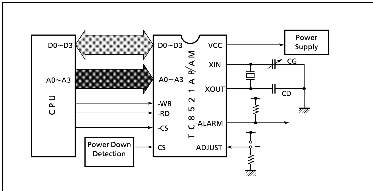
FIG.3.2 SYSTEM CONFIGURATION
