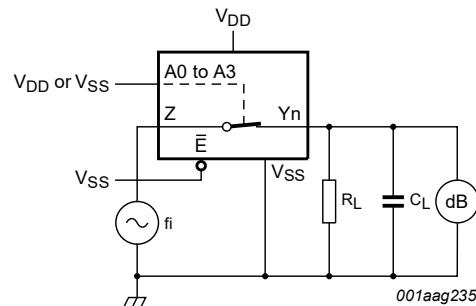
Fig. 13. Test circuit for measuring frequency response
