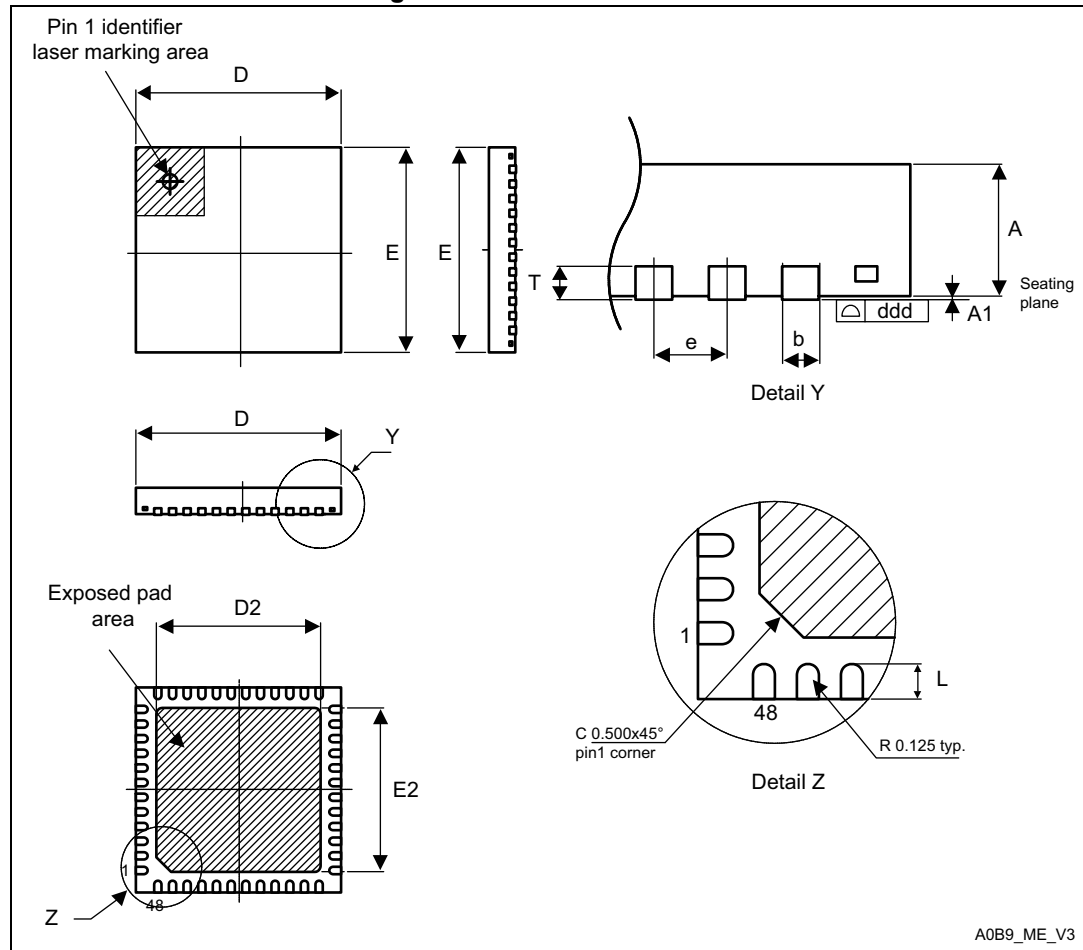
Figure 78. UFQFPN48 outline
