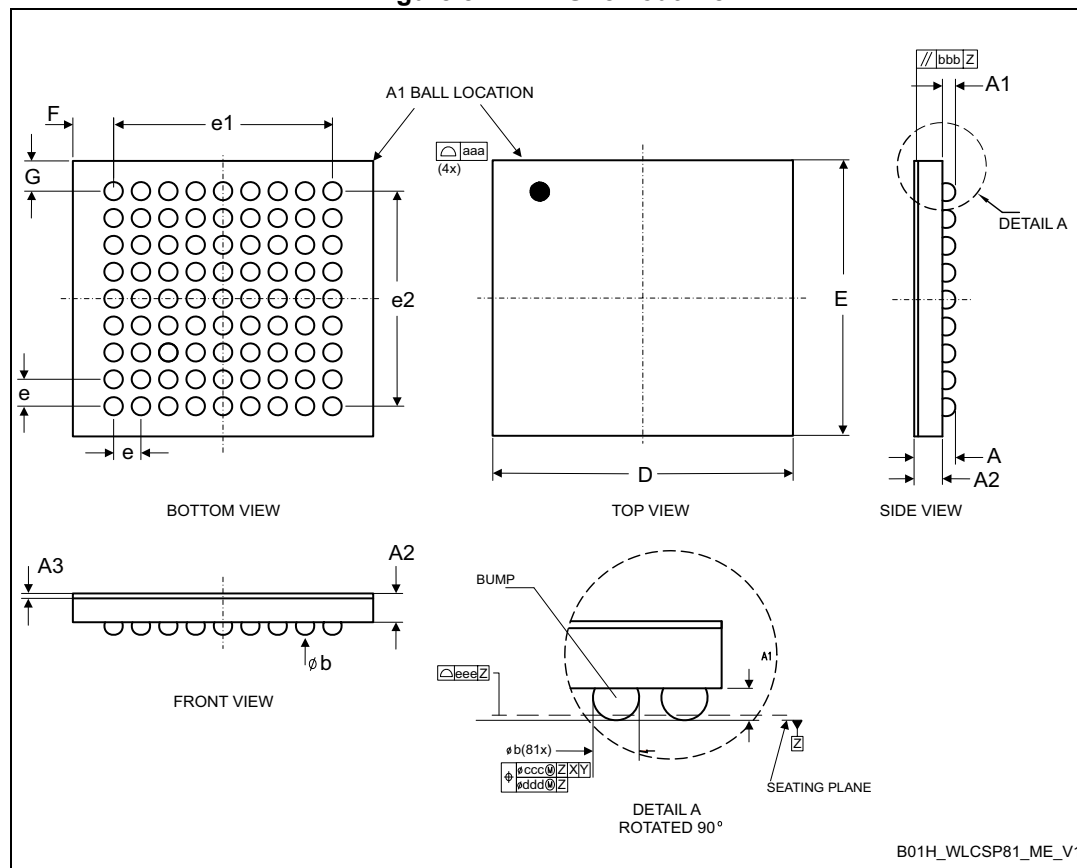
Figure 82. WLCSP81 outline
