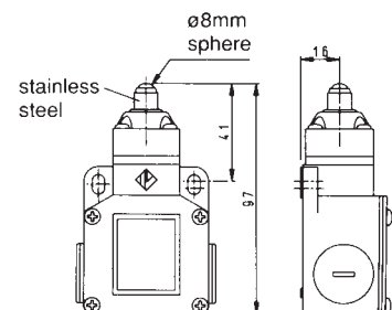
Actuator type 18 Rolling ball piston plunger
