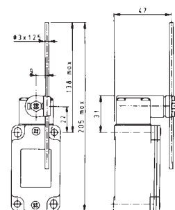
Actuator type 32 Adjustable round steel rod lever
