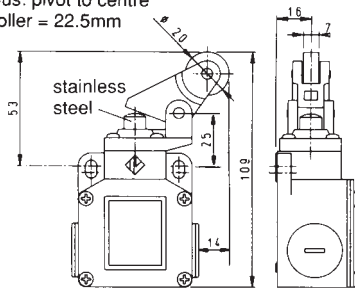
Actuator type 05 One-way roller - side actuated
