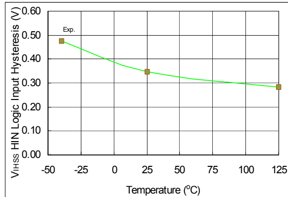
Figure 33. V IHSS HIN Logic Input Hysteresis vs. Temperature
