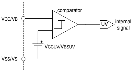
Figure 1: Undervoltage Diagram
