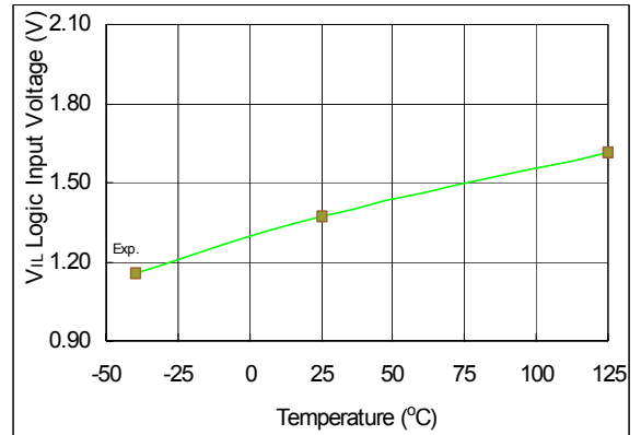
Figure 32. V IL Logic Input Voltage vs. Temperature
