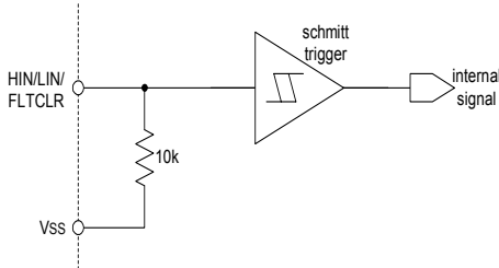
Figure 2: HIN, LIN and FLTCLR Diagram
