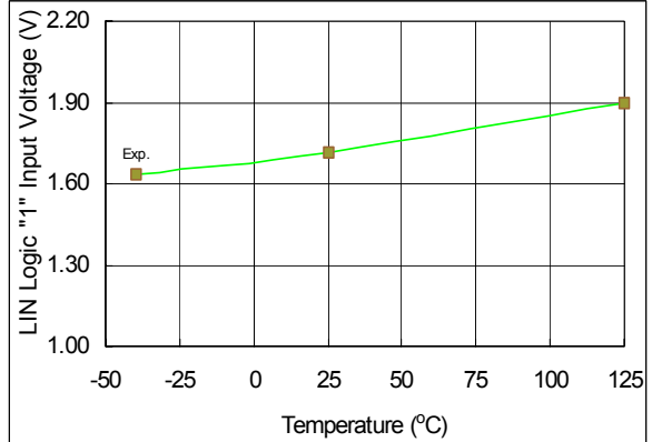
Figure 34. LIN Logic "1" Input Voltage vs. Temperature
