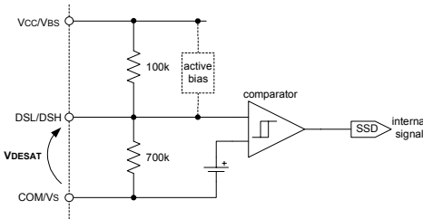
Figure 4: DSH and DSL Diagram
