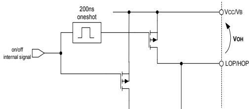
Figure 5: HOP and LOP Diagram
