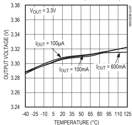
OUTPUT VOLTAGE vs. TEMPERATURE (BUCK MODE)
