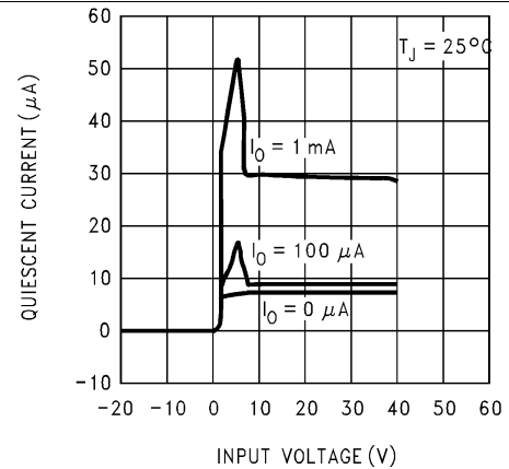
Figure 4. Quiescent Current
