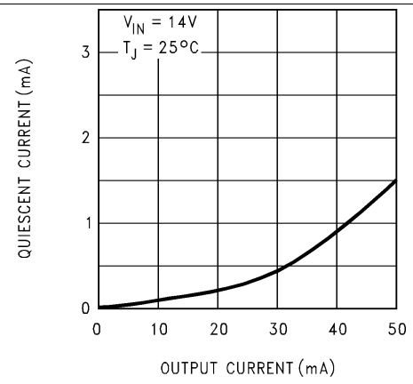
Figure 6. Quiescent Current
