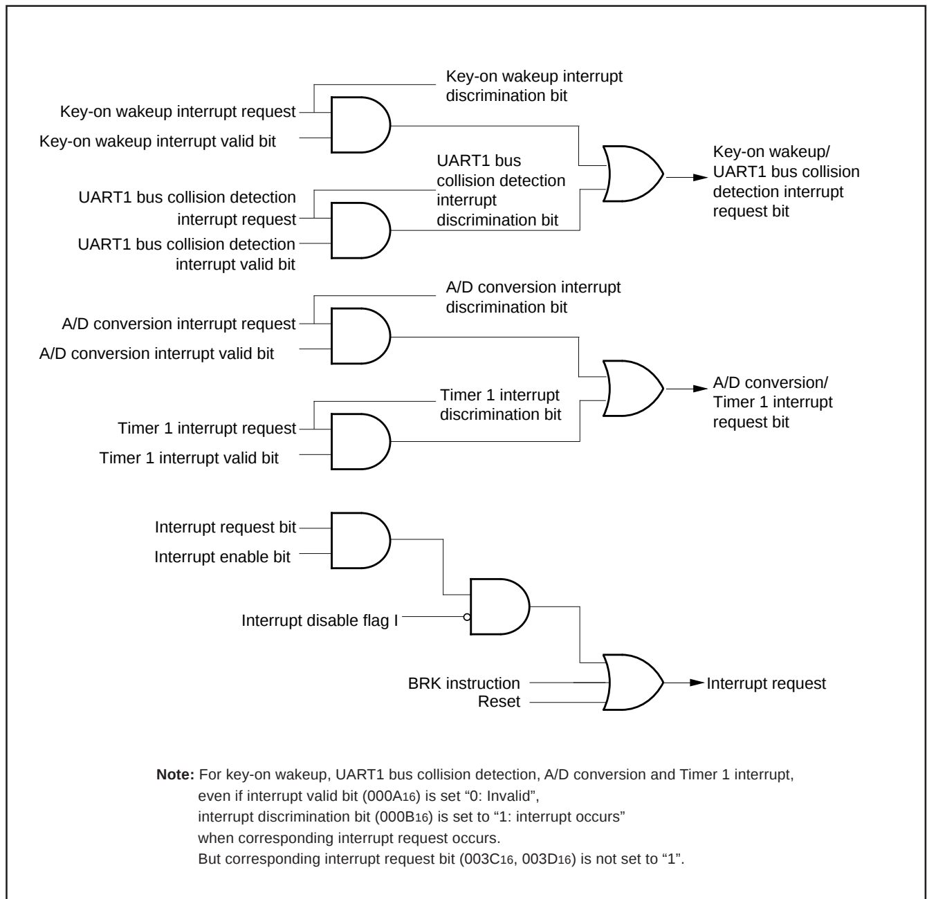
Fig. 23 Interrupt control
