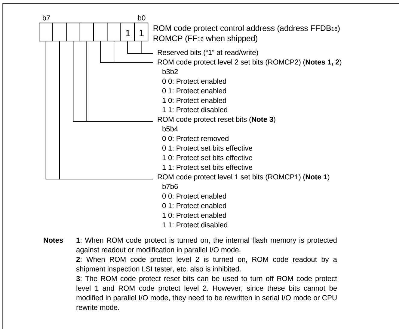
Fig. 102 Structure of ROM code protect control address
