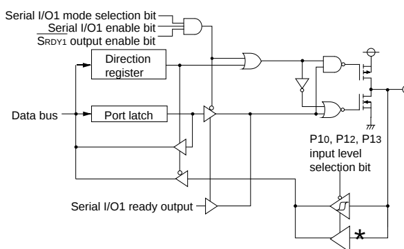
(11) Port P1 3
