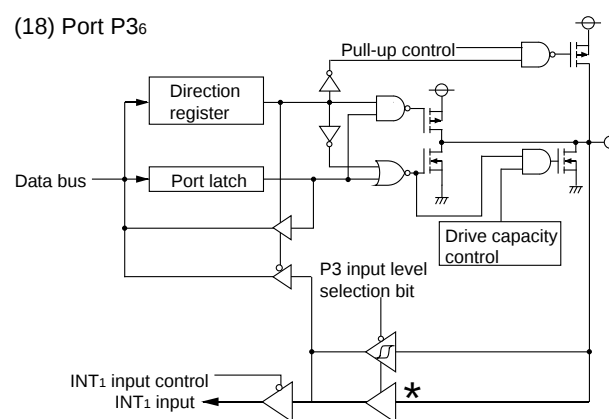
(19) Port P3 7
