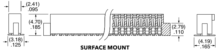
SURFACE MOUNT
