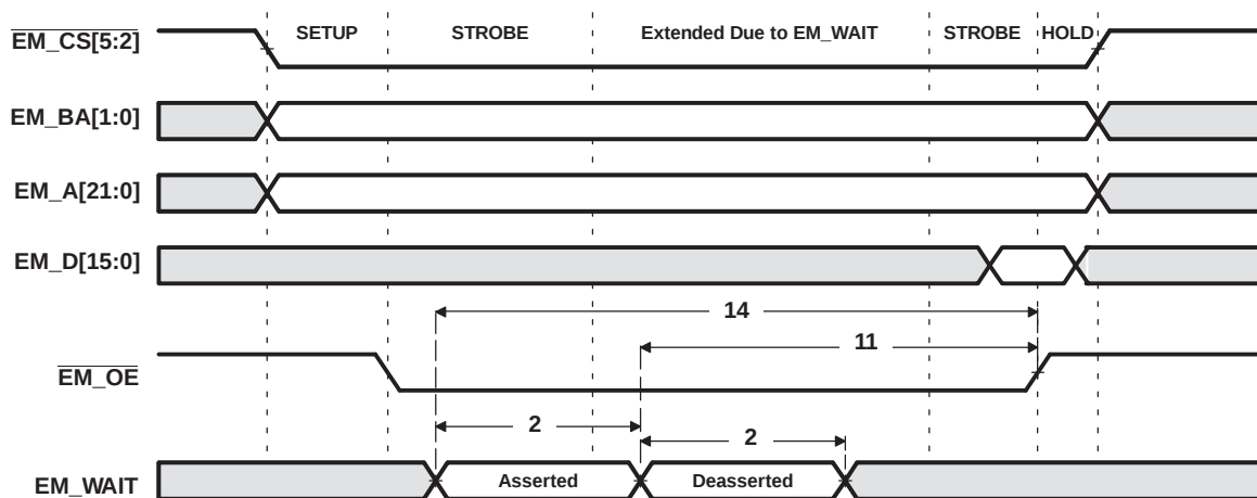
Figure 6-23. \text{EM\_WAIT} Read Timing Requirements
