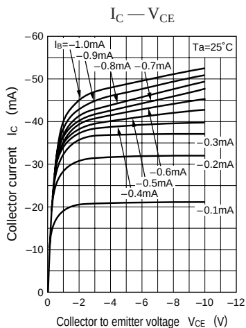
Characteristics charts of UN111E
