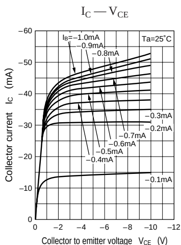
Characteristics charts of UN111D
