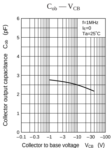
Characteristics charts of UN111E
