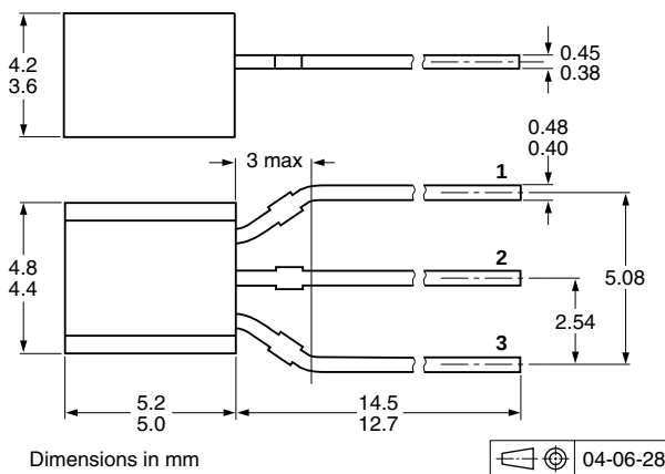
Fig 5. Package outline SOT54A
