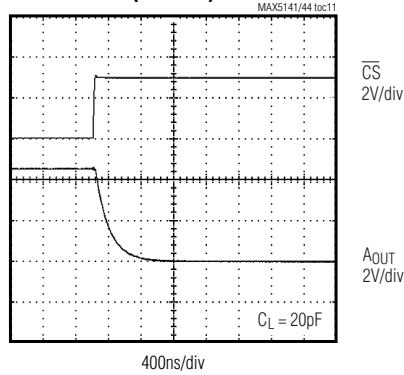
FULL-SCALE STEP RESPONSE (FALLING)
