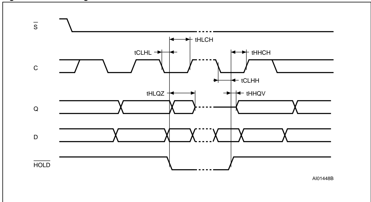
Figure 16. Hold Timing
