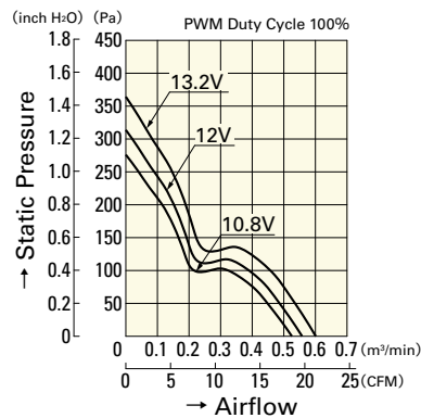
9WL0412P3G001
