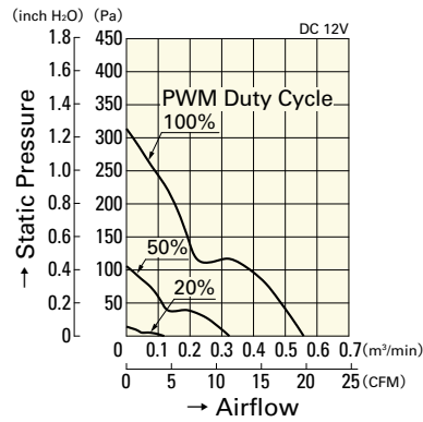
9WL0412P3G001
