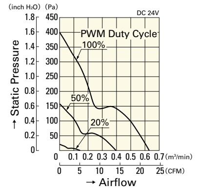
9WL0424P3J001
