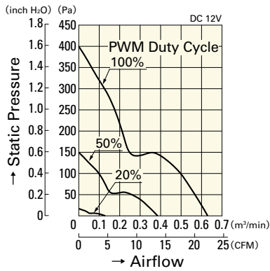
9WL0412P3J001
