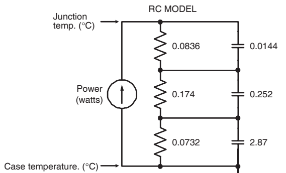
FIGURE 19b, TRANSIENT THERMAL IMPEDANCE MODEL
