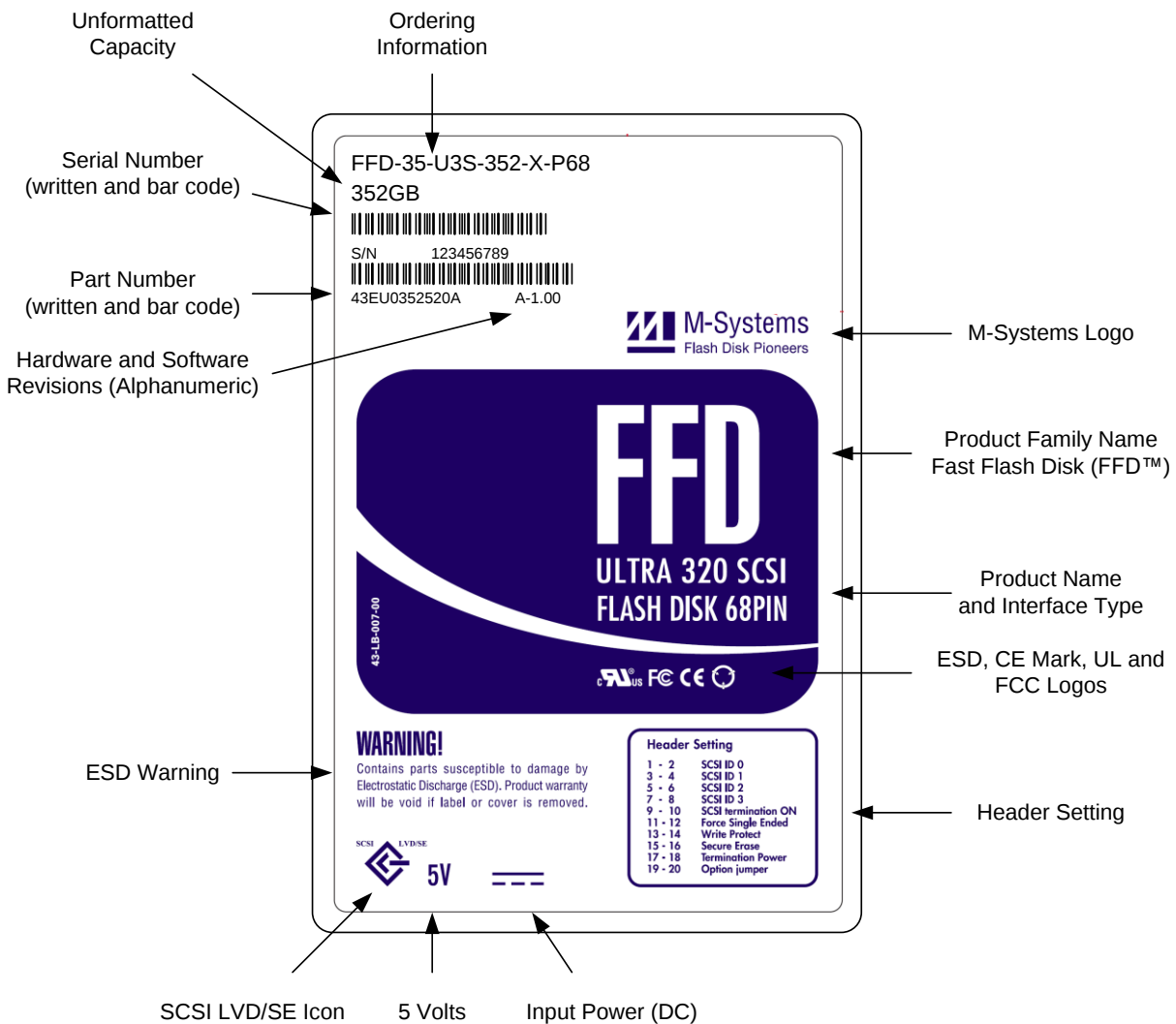
Figure 15: SSD Ultra320 SCSI 3.5" 68-Pin Label
