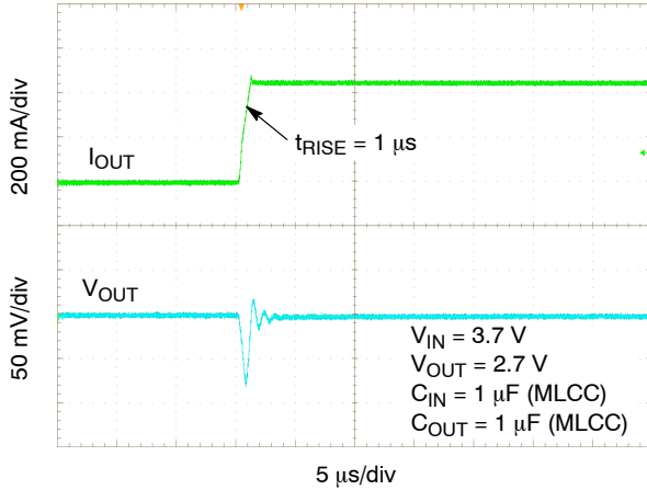
Figure 33. Load Transient Response – 1 mA to 450 mA – V_{OUT} = 2.7 V
