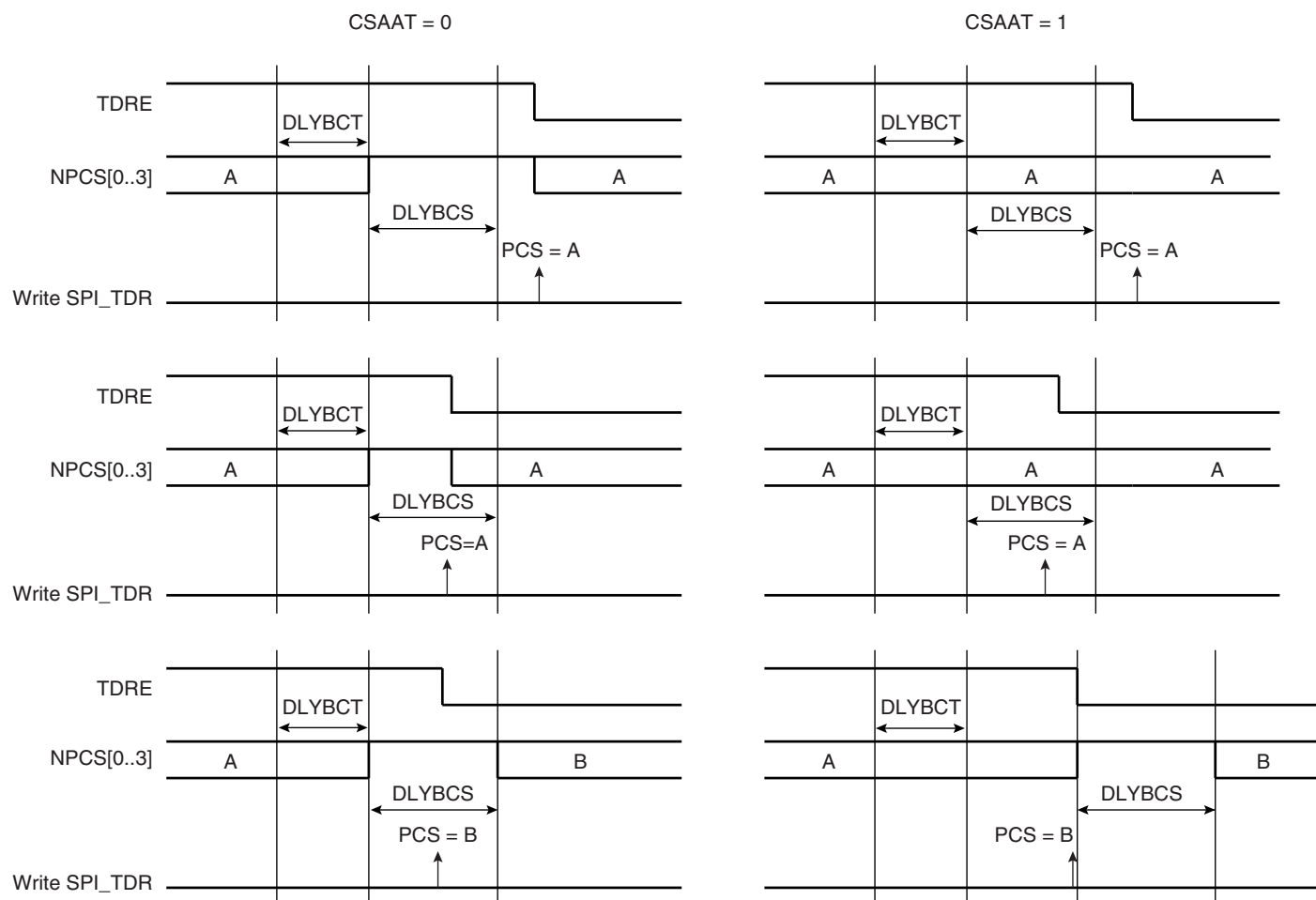
Figure 29-8. Peripheral Deselection
