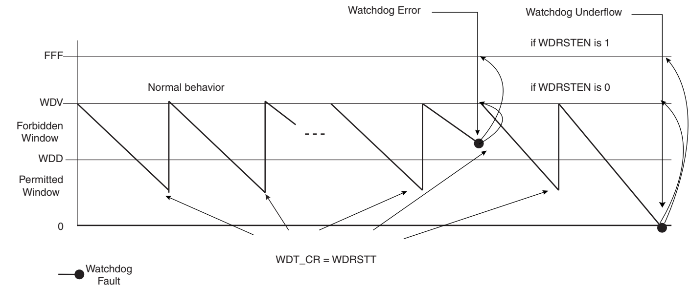
Figure 15-2. Watchdog Behavior
