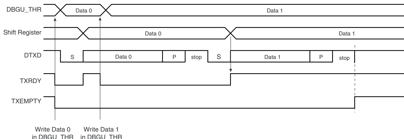
Figure 27-11. Transmitter Control
