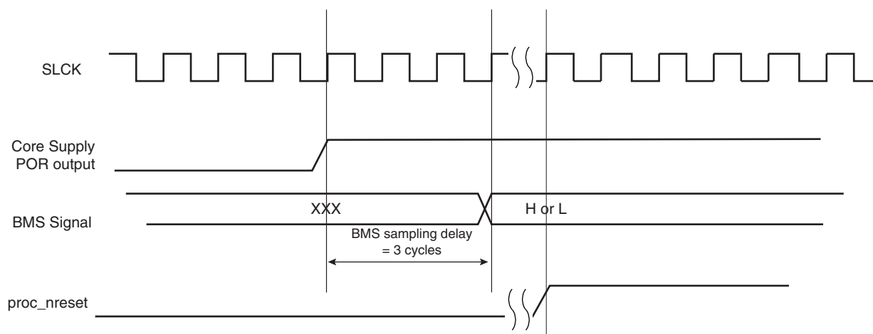
Figure 12-3. BMS Sampling
