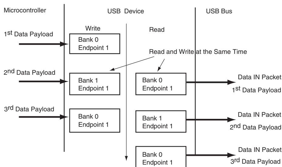
Figure 36-7. Bank Swapping Data IN Transfer for Ping-pong Endpoints
