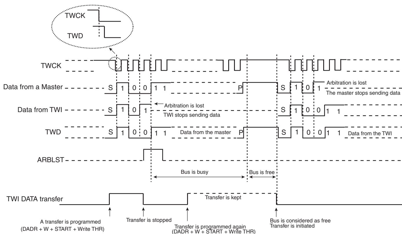
Figure 30-21. Arbitration Cases
