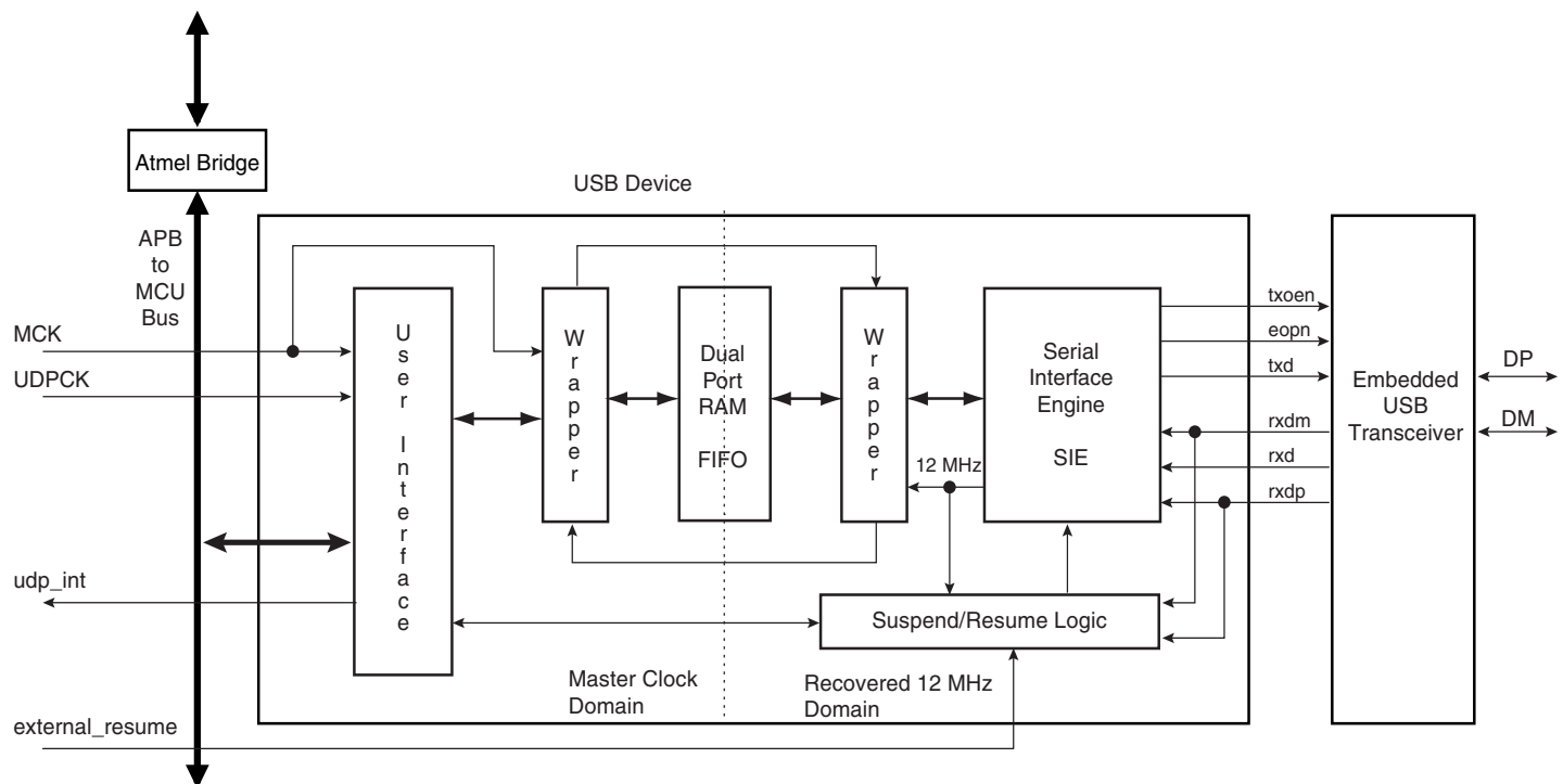
Figure 36-1. Block Diagram
