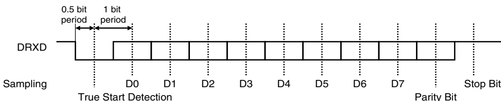
Figure 27-5. Character Reception
