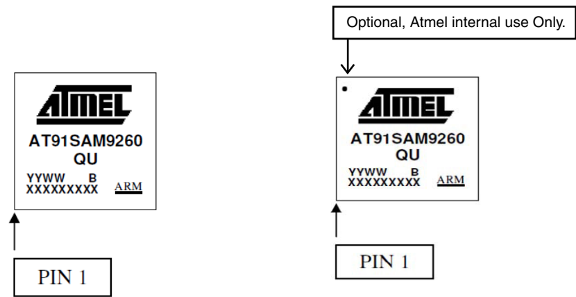
Figure 41-3. 208-lead PQFP: Pin 1 Position
