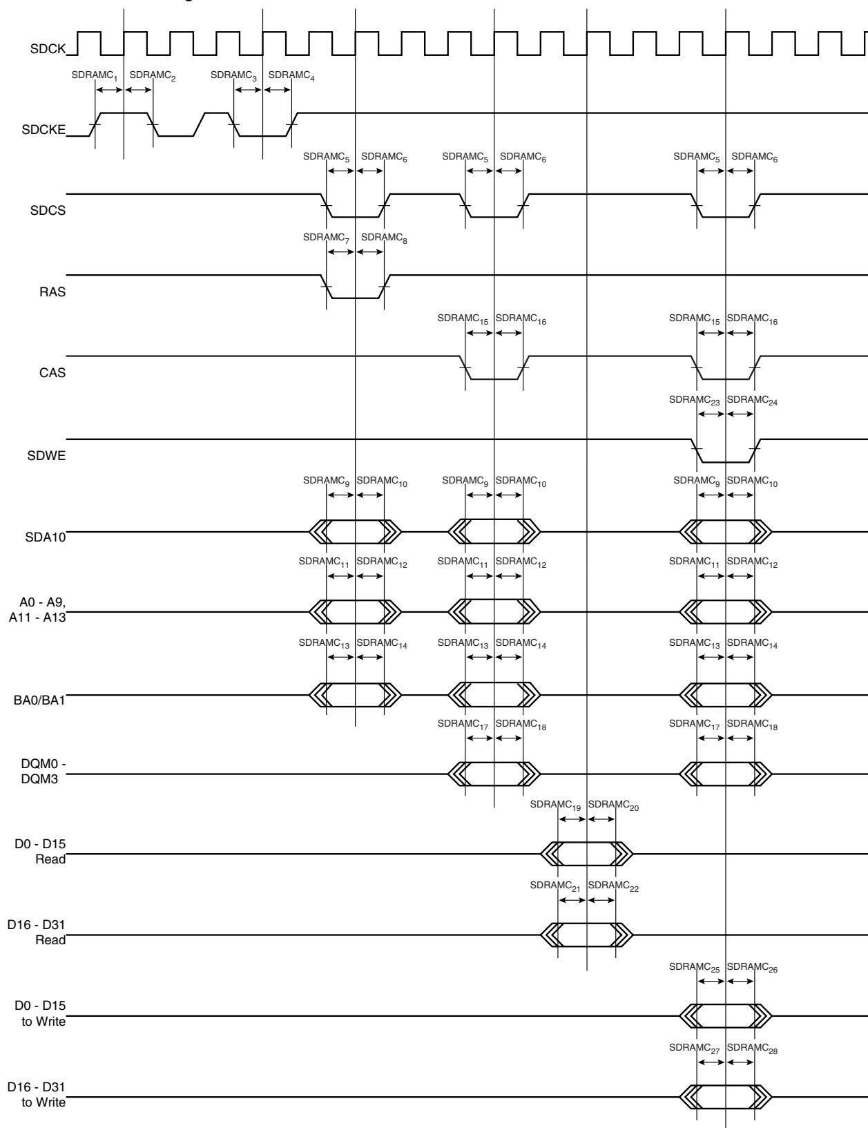
Figure 40-5. SDRAMC Signals Relative to SDCK
