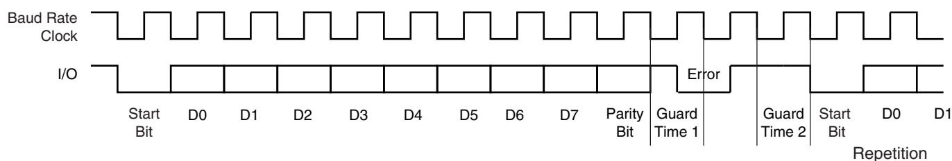
Figure 31-22. T = 0 Protocol with Parity Error
