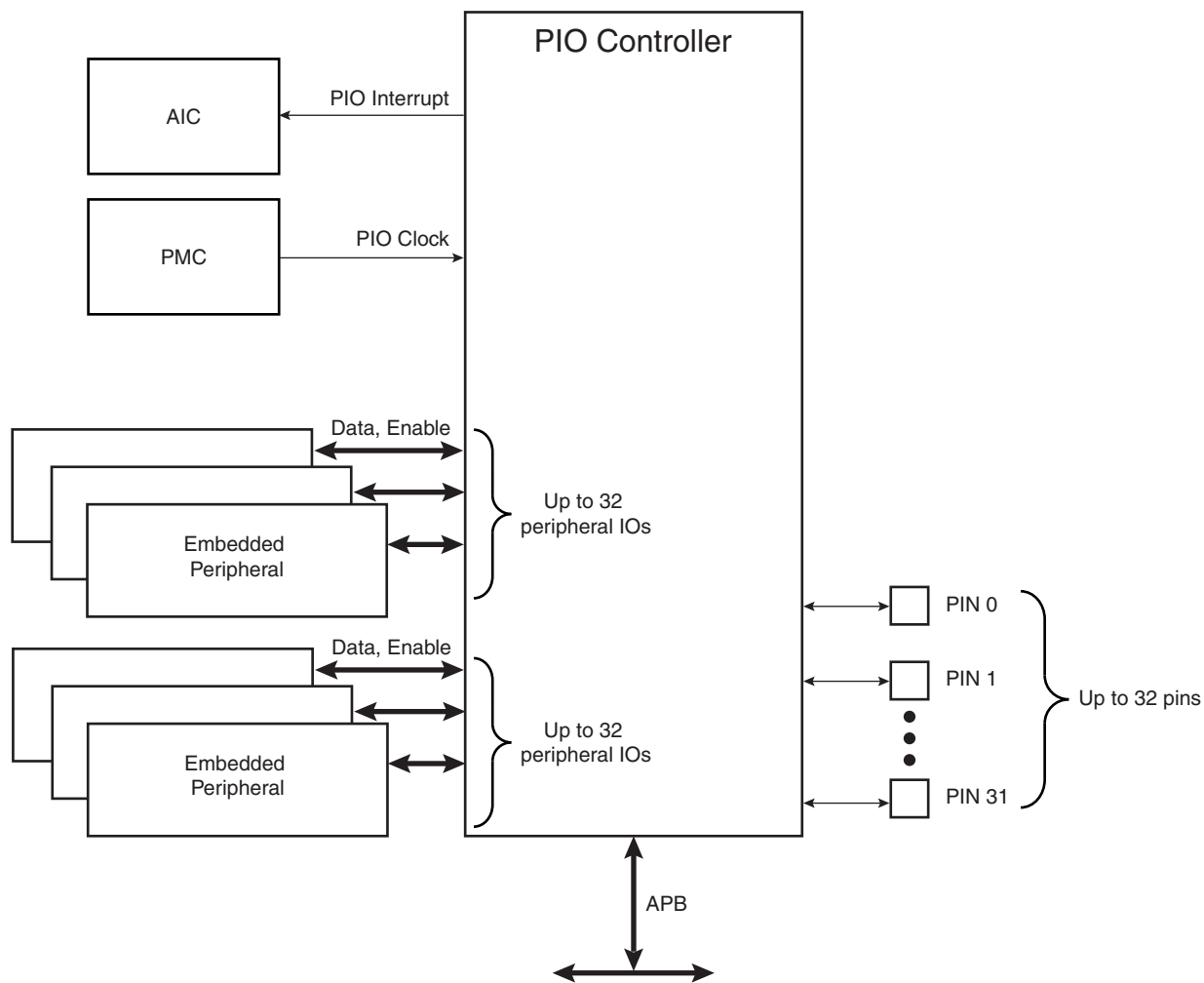
Figure 28-1. Block Diagram
