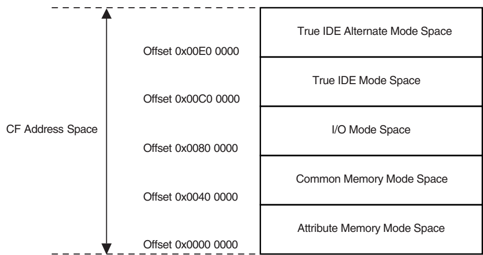
Figure 19-3. CompactFlash Memory Mapping
