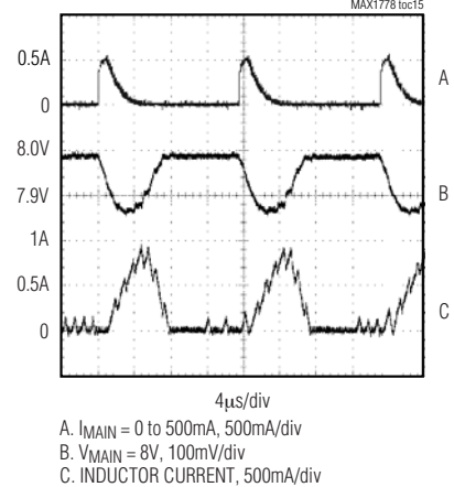
STEP-UP CONVERTER LOAD-TRANSIENT RESPONSE (1uS PULSES)
