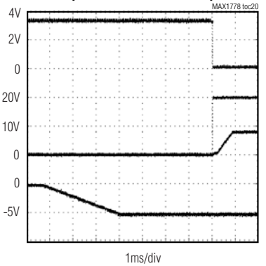
POWER-UP SEQUENCE (CIRCUIT OF FIGURE 10)
