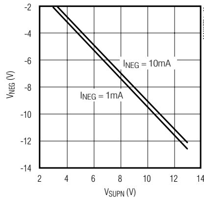
MAXIMUM NEGATIVE CHARGE-PUMP OUTPUT VOLTAGE vs. SUPPLY VOLTAGE
