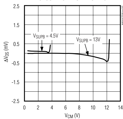
INPUT OFFSET VOLTAGE DEVIATION vs. COMMON-MODE VOLTAGE
