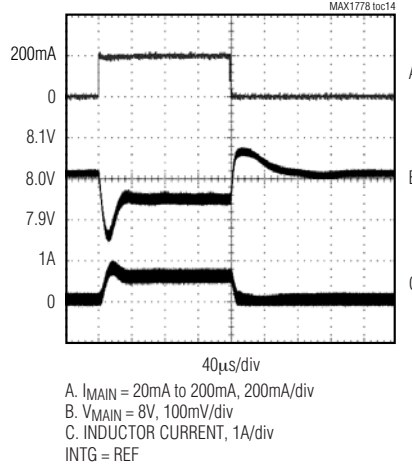
STEP-UP CONVERTER LOAD-TRANSIENT RESPONSE WITHOUT INTEGRATOR
