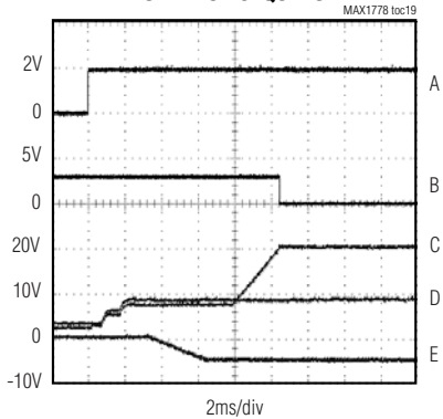
POWER-UP SEQUENCE
