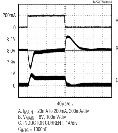
STEP-UP CONVERTER LOAD-TRANSIENT RESPONSE
