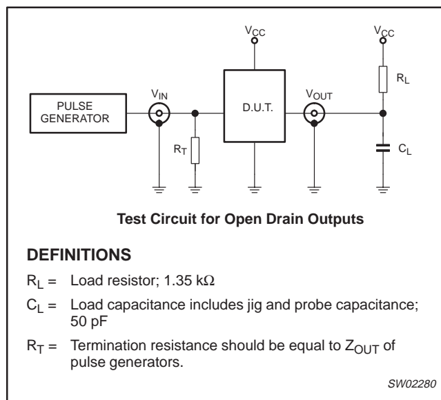
Figure 7. Test circuit
