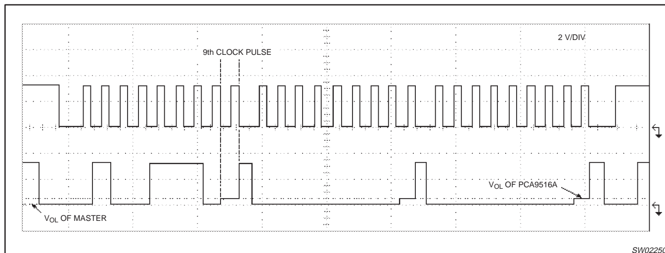
Figure 5. Bus 0 waveform
