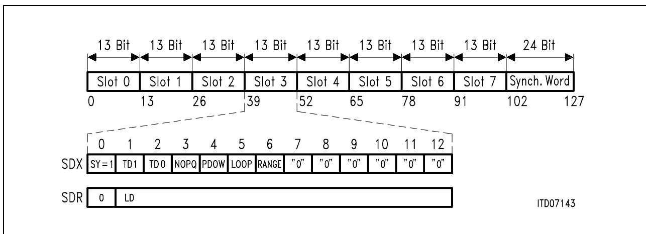
Figure 9 Frame Structure on SDX and SDR in 4B3T Mode
