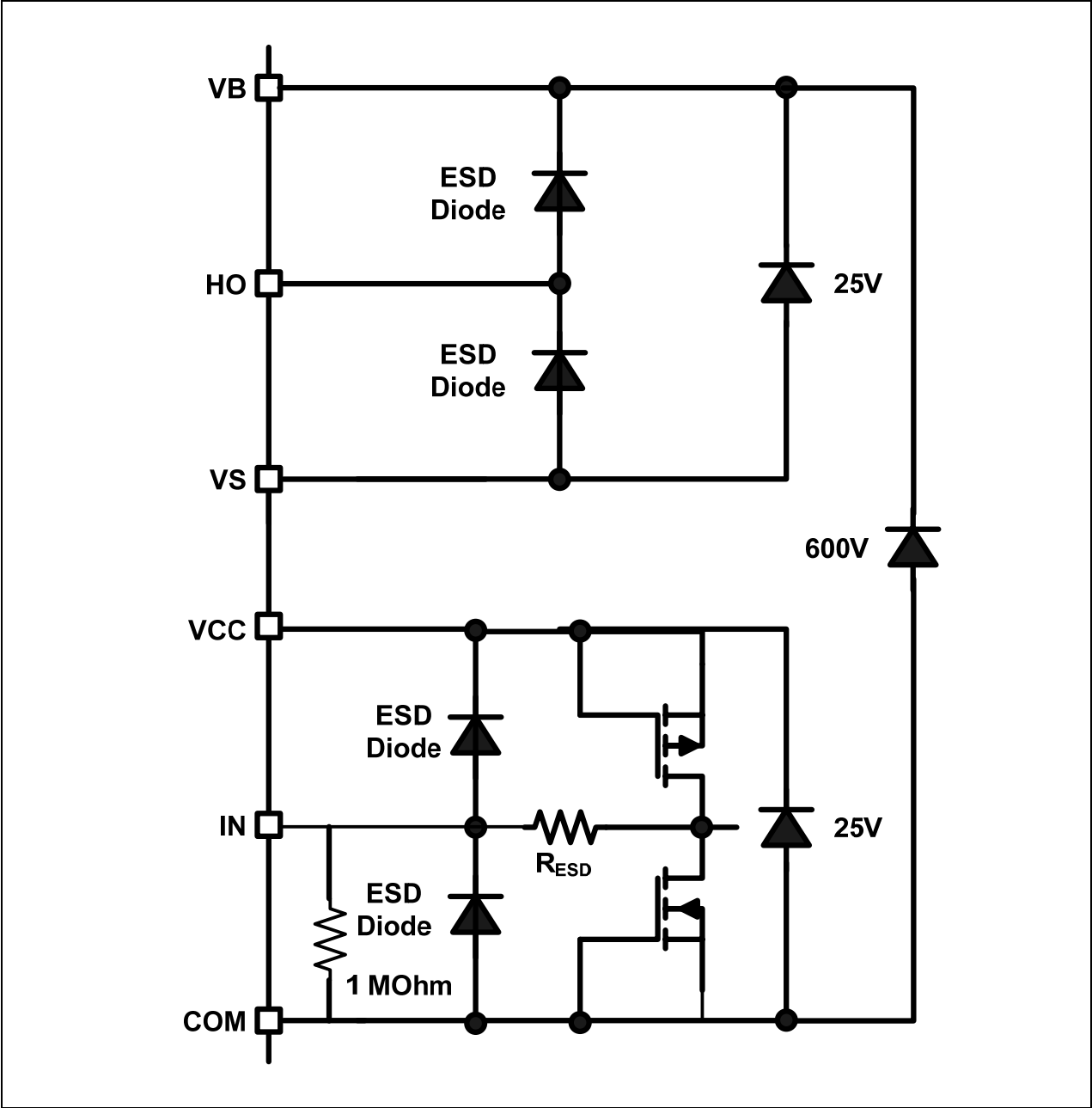
I/O Pin Equivalent Circuit Diagram
