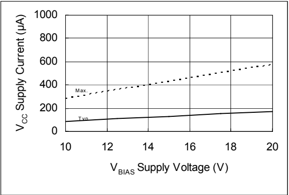
Figure 9B. Vcc Supply Current vs. Supply Voltage
