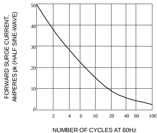
Fig. 4-NON-RECURRENT SURGE RATING
