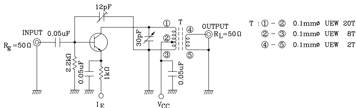
Fig. G_{pe} TEST CIRCUIT
