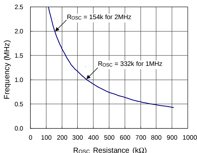
Figure 1. Switching Frequency vs. ROSC Resistance
